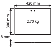
Single Leg Base 8 mm RAL 9006 Powdercoated aluminium base
